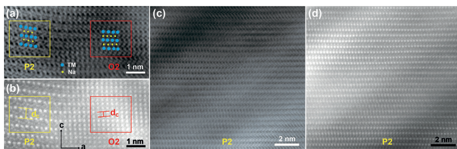
Figure 4. a) ABF- and b) HAADF-STEM images of a P2-type \text{Na}_{0.67}\text{Mn}_{0.67}\text{Ni}_{0.33-x}\text{Mg}_x\text{O}_2 ( x=0 ) electrode when charging to 4.22 V at the [010] zone axis; the yellow and red rectangles indicate areas with the P2 and O2 structure. c) ABF- and d) HAADF-STEM images of a P2-type \text{Na}_{0.67}\text{Mn}_{0.67}\text{Ni}_{0.33-x}\text{Mg}_x\text{O}_2 ( x=0.05 ) electrode when charging to 4.22 V.
